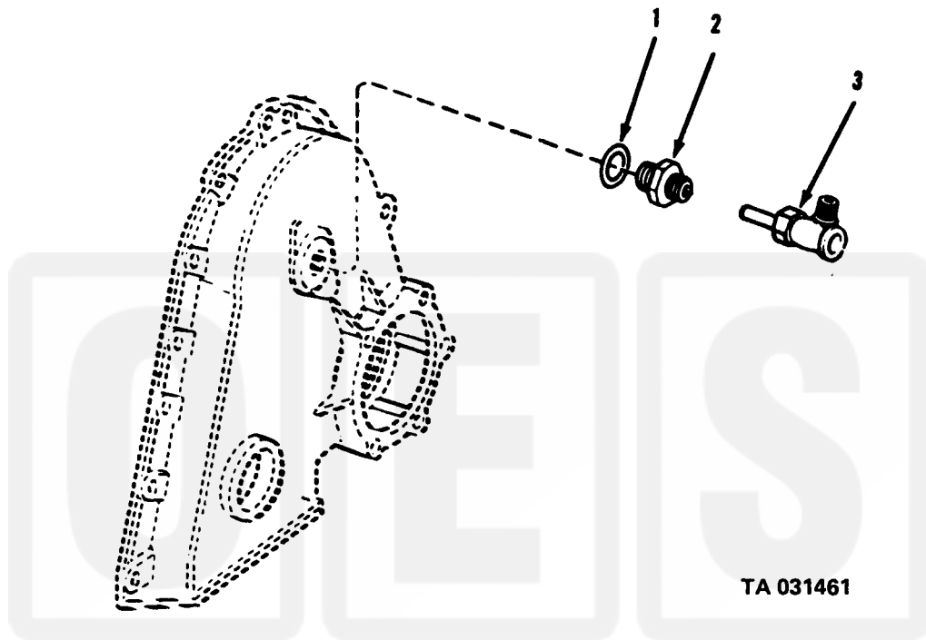
Figure 345. Tachometer drive and take-off adapter.
